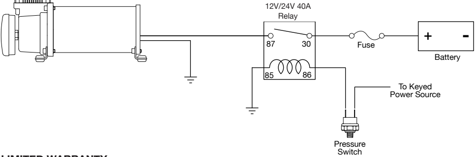
(Fig. 4) Recommended Wiring Diagram: (Fuse Not Included)
